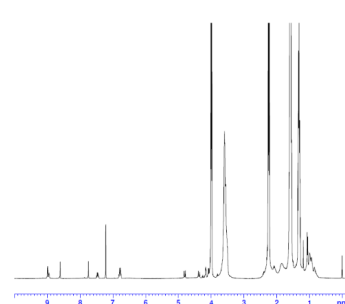
Fig.4 1 H-NMR
