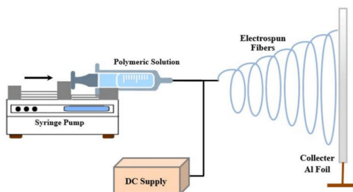
Figure 2. Electrospinning technique
