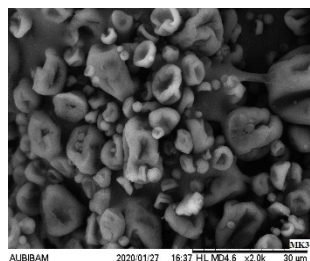
Figure 1: SEM microimage
